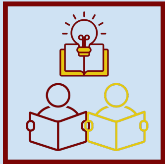
Learning Rep
