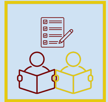
Testing Rep
